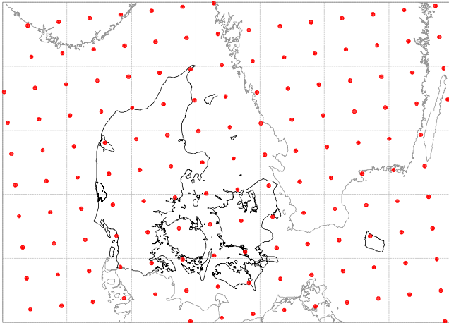
Figure 1 Resolution of applied climate model data provided by Max Plank Institute in Germany
