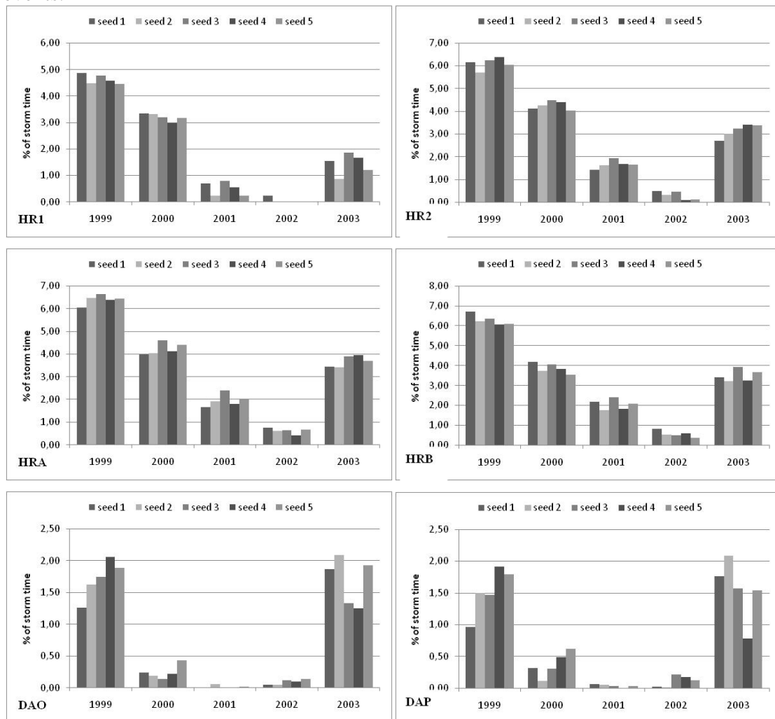
Figure 19 Loss of production as percentage of total storm time; SST control
