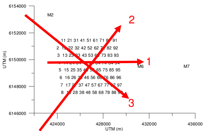
Figure 3: Horns Rev layout including definition of Case 1 ( 7D ), Case 2 ( 9.4D ) and Case 3 ( 10.5D ) flow directions. Turbine locations are given by numbers and the location of the downstream masts are marked with M6 and M7.
