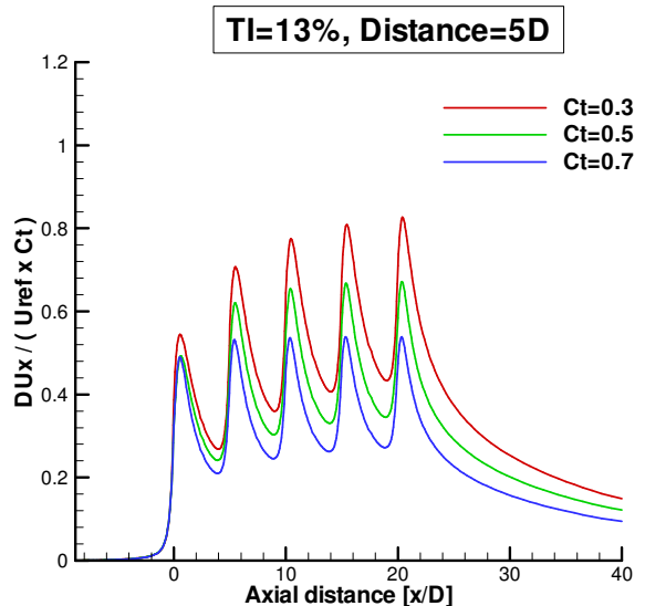
Figure 2: CFD simulations of five wind turbines in flat terrain - Effect of C_t on velocity deficit at hub height. Distance between wind turbines is 5D and inlet turbulence intensity at hub height is 13%.
